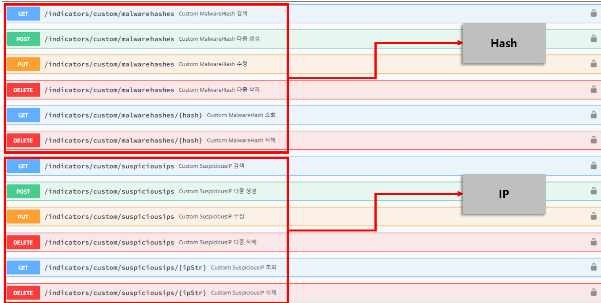
Fig. 2: Genian EDR REST API
